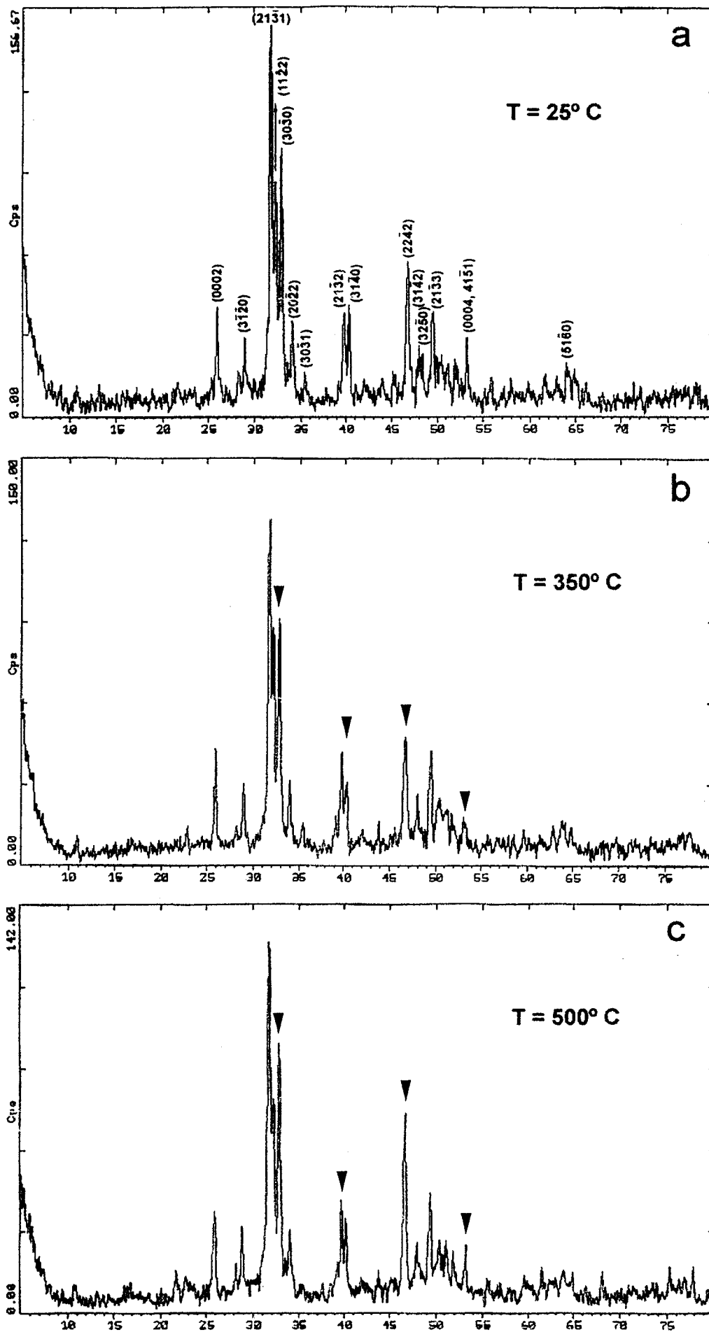
Figure 1 X-ray diffractograms from the in situ heating experiments in air of a powder enamel sample: (a) at room temperature, (b) at 350°C, and (c) at 500°C. The indexation fit very well with the hexagonal structure of hydroxyapatite. Note that the only difference is the change in intensity of some peaks, mainly those marked.
